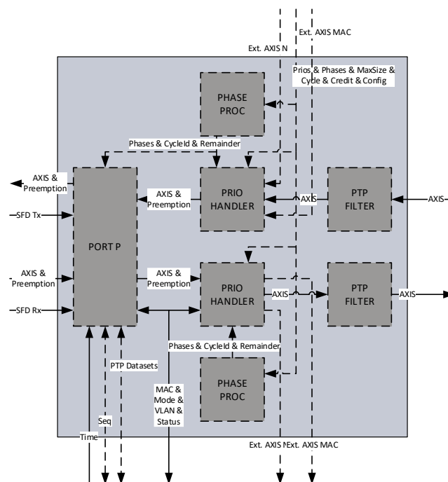
Figure 17: Port E
