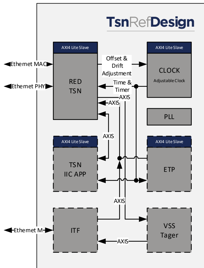
Figure 27: Reference Design
