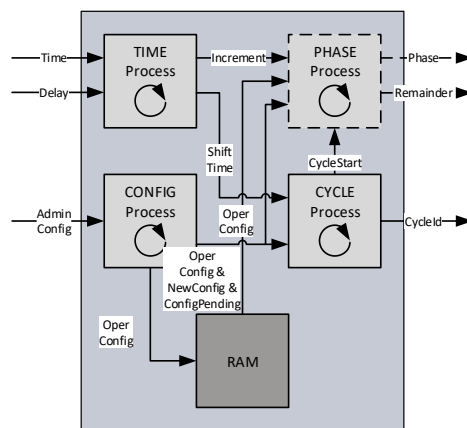
Figure 20: Phase Processor
