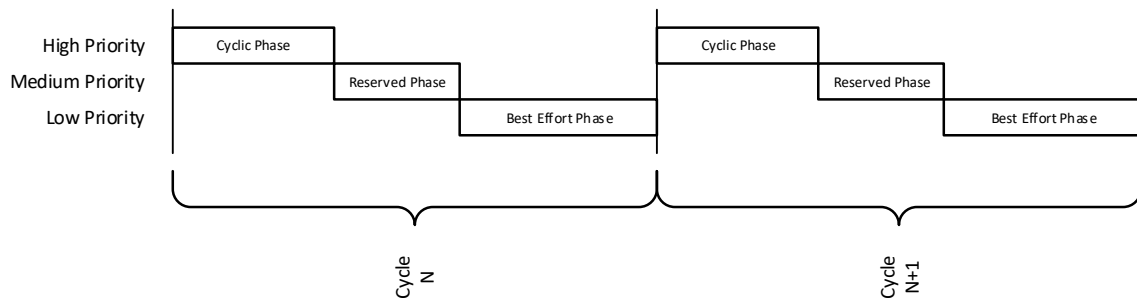
Figure 10: Simple Schedule
