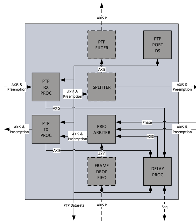
Figure 18: Port P
