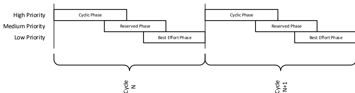
Figure 11: Overlapping Schedule
