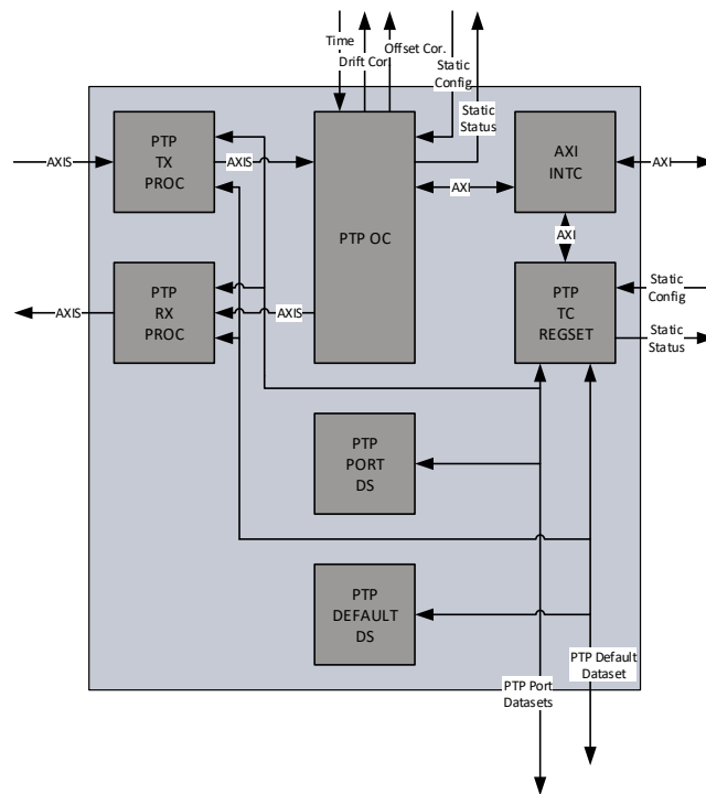
Figure 21: PTP Processor
