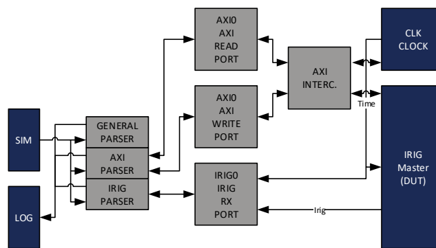
Figure 11: Testbench Framework
