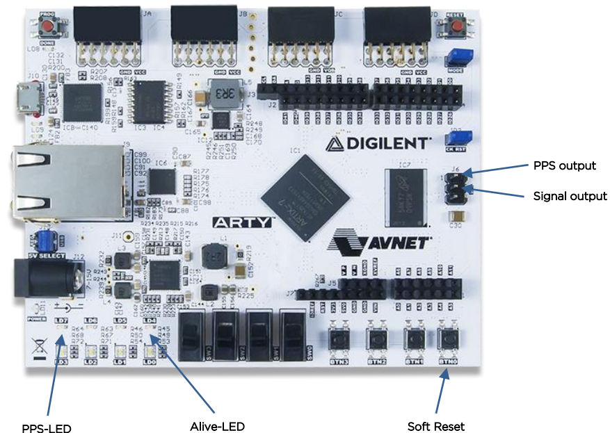
Figure 13: Arty (source Digilent Inc)
